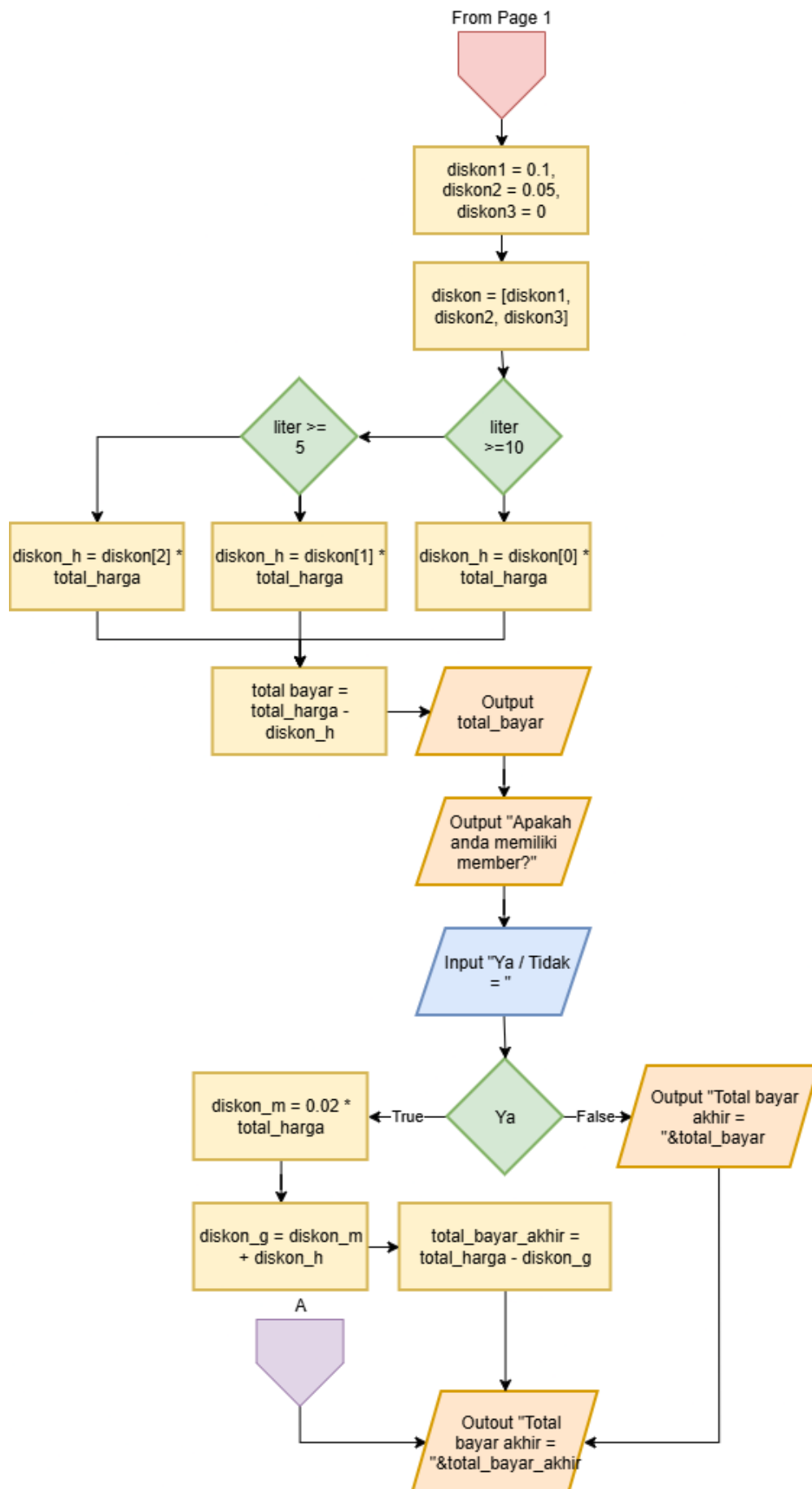
Gambar 1.2 Desain Flowchart
