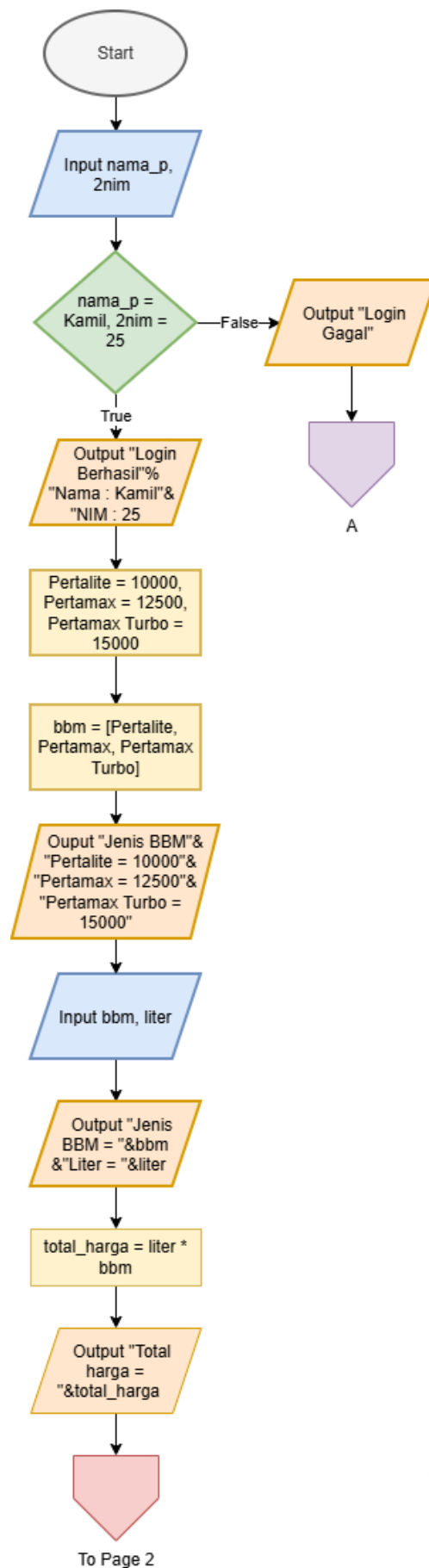
Gambar 1.1 Desain Flowchart
